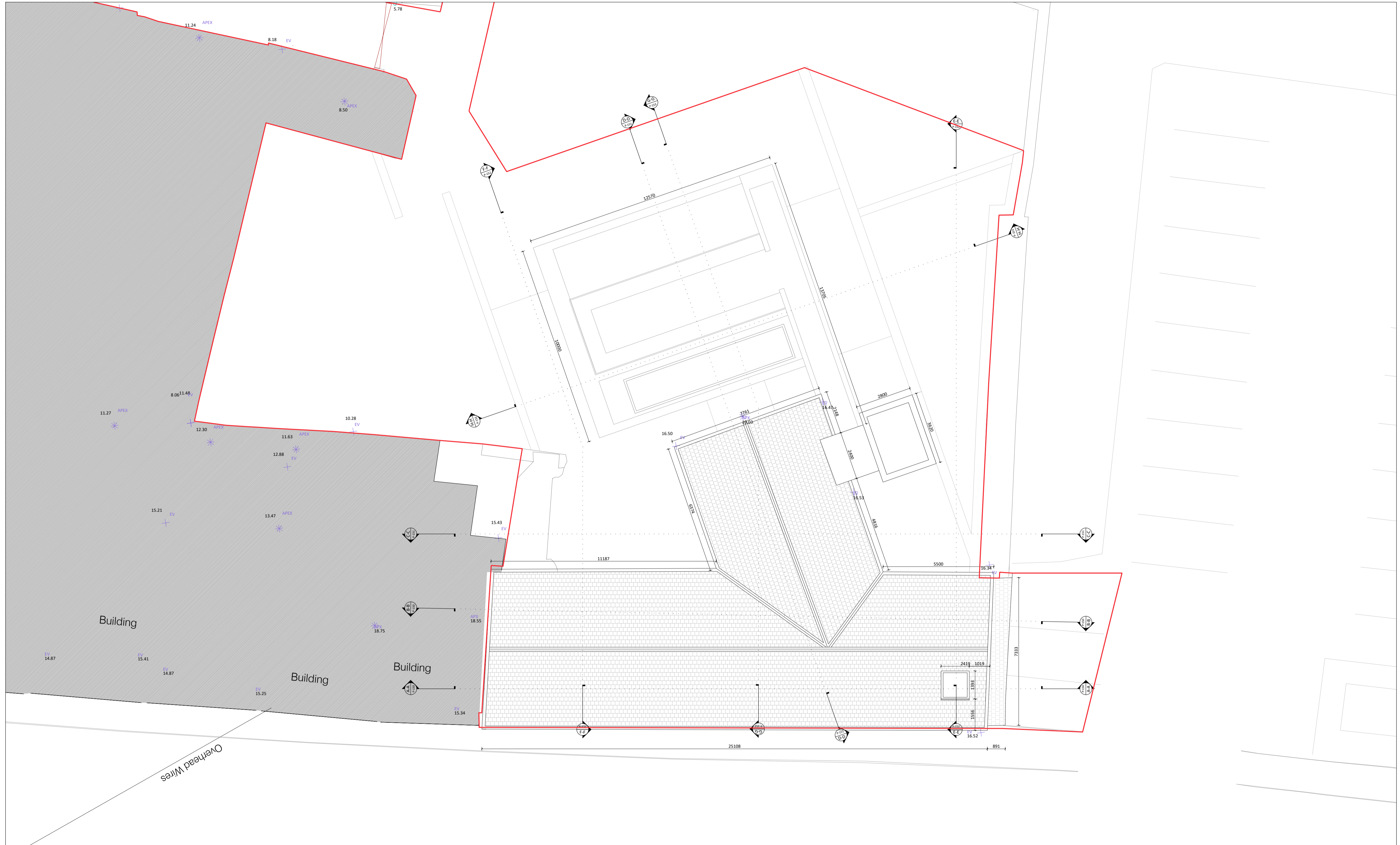
01 Roof Plan As Proposed Scale: 1:100
